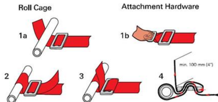
Proper Wrapping of a Shoulder Belt
