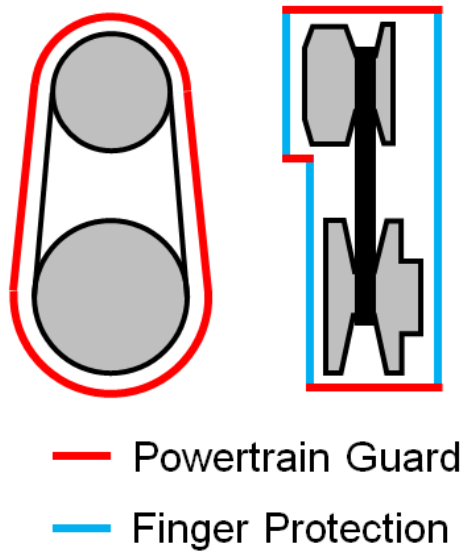
Figure B-54: Powertrain Guard Extent example on a CVT
