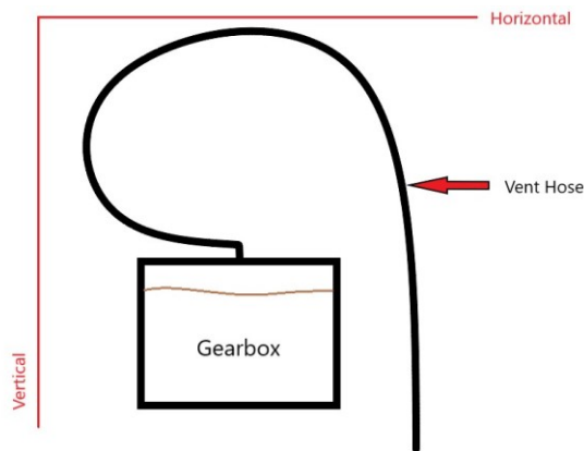
Figure B-57: Air Trap Vent Line Routing
