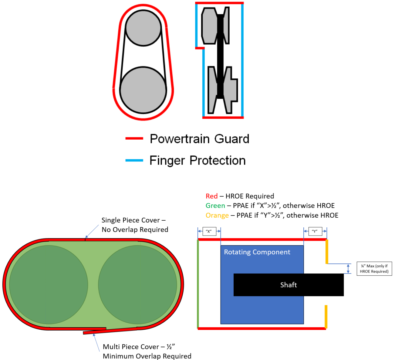
Figure B-49: Powertrain Guard Extent example on a CVT
