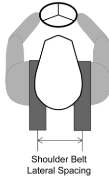
Figure B-32: Driver Harness, Shoulder Harness Lateral Position, Overhead view
