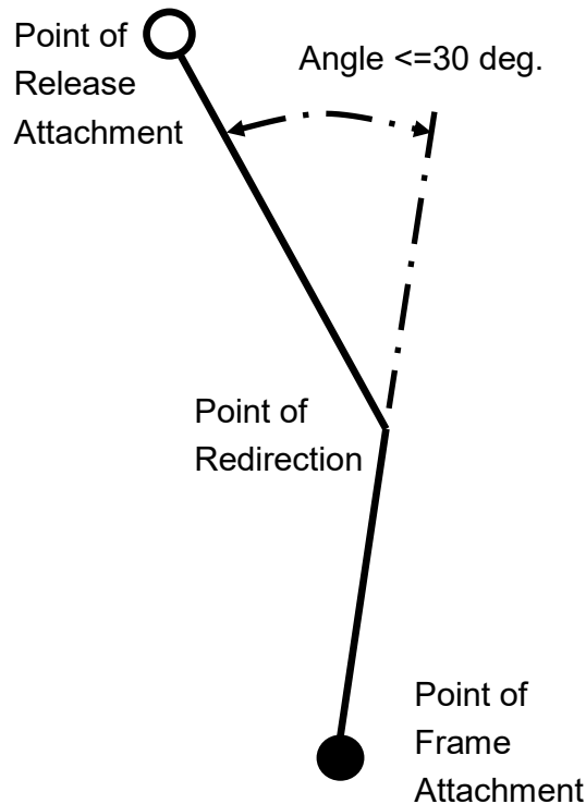
Figure B-37: Driver Harness, Anti-Submarine Belt Redirection
