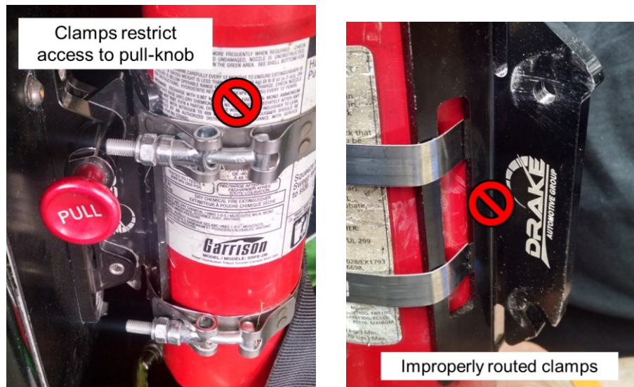
Figure B-48: Incorrect orientation of extinguisher clamps.
