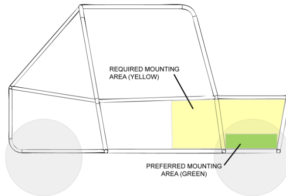
Figure B-61: Transponder, Mounting Location
