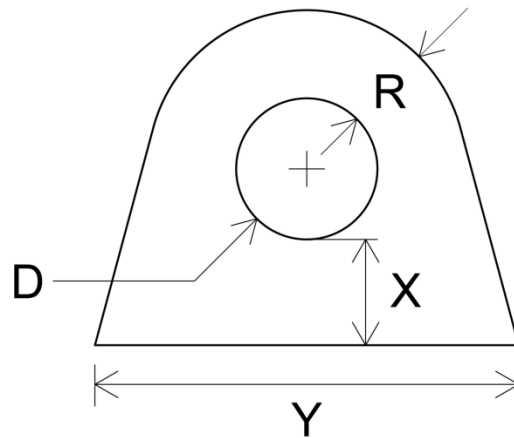
Figure B-55: Tow Point, Rear Tab Dimensions
