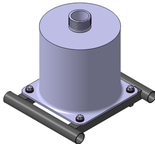
Figure B-43: Fuel tank mounted to square/rectangular tubes (preferred mounting design)
