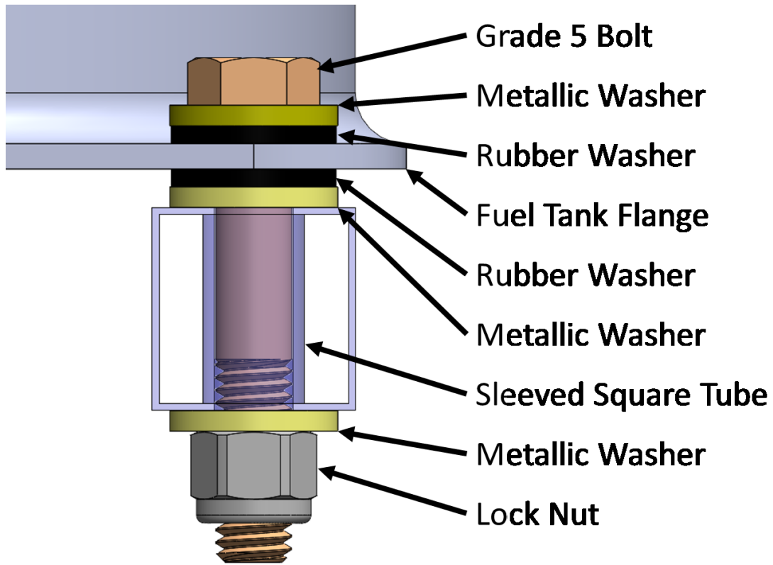
Figure B-42: Fuel Tank Fastener Stack-up
