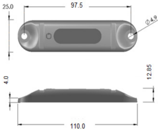
Figure B-64: RFID Tag Dimensions
