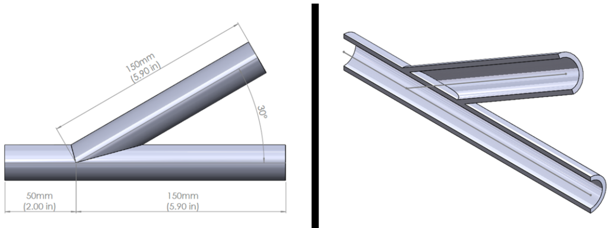
Figure B-27: Roll Cage, Welding Sample 2
