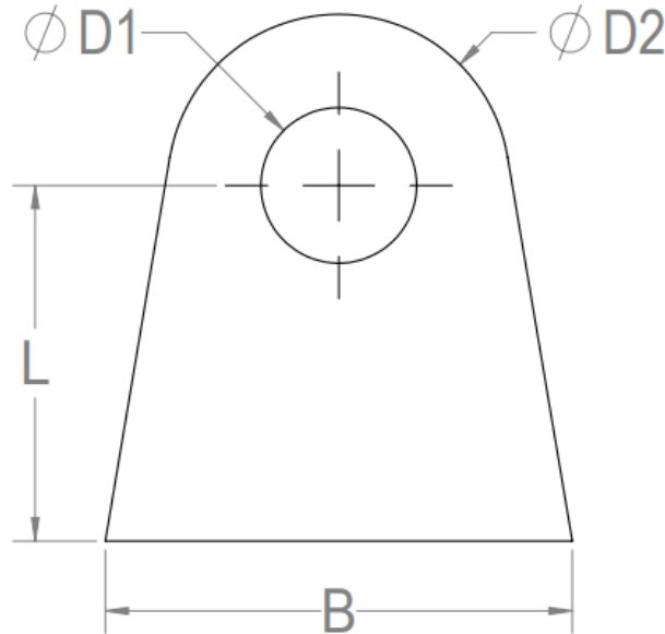
Figure B-57: Required Tab Drawing
