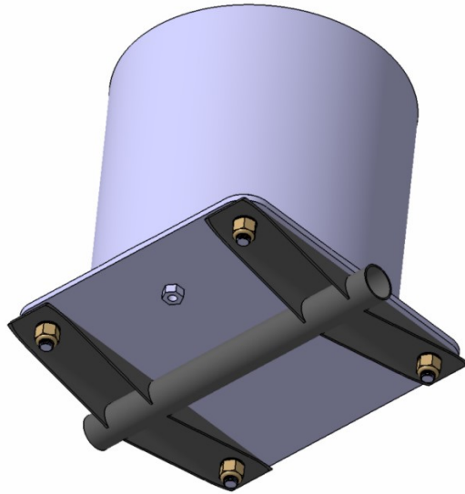
Figure B-44: Fuel tank mounted to "C" brackets. (Acceptable mounting design)
