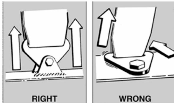
Figure B-36: Driver Harness, Lap Belt Tab Orientation
