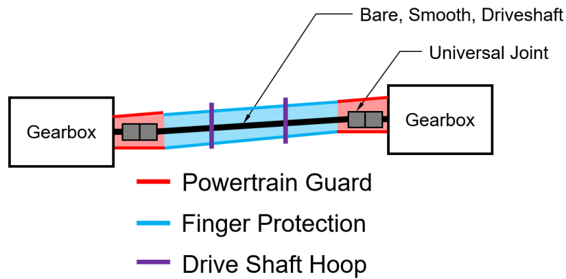
Figure B-50: Driveshaft Guarding
