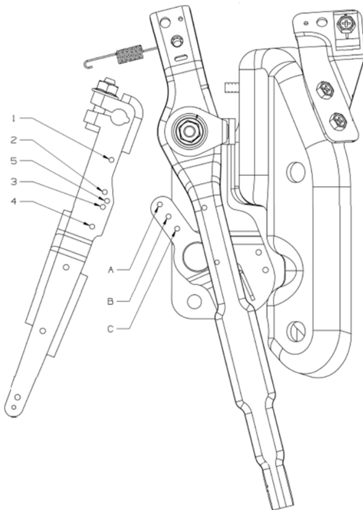
Figure B-1: Engine Governor
